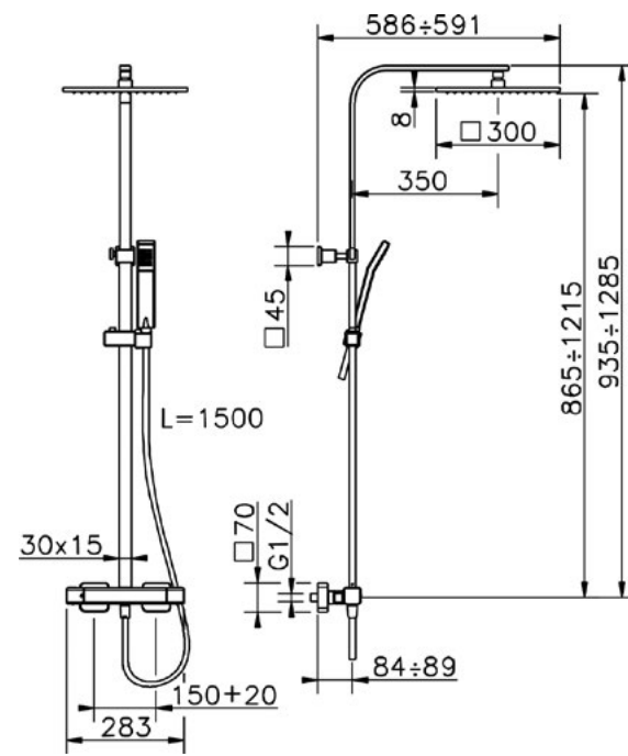
CU C8601M CombiDoccia Termostatico Thermo CombiShower CombiDouche Thermo
