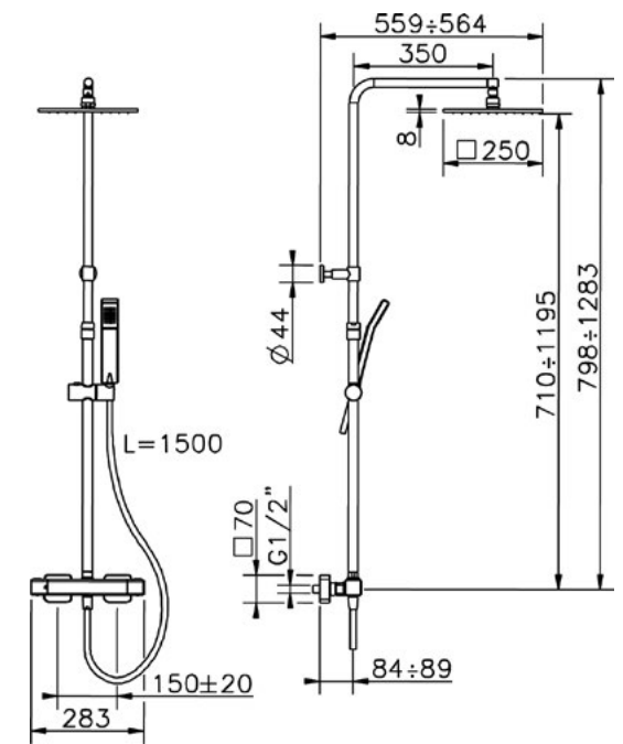
CU C8401C CombiDoccia Termostatico Thermo CombiShower CombiDouche Thermo
