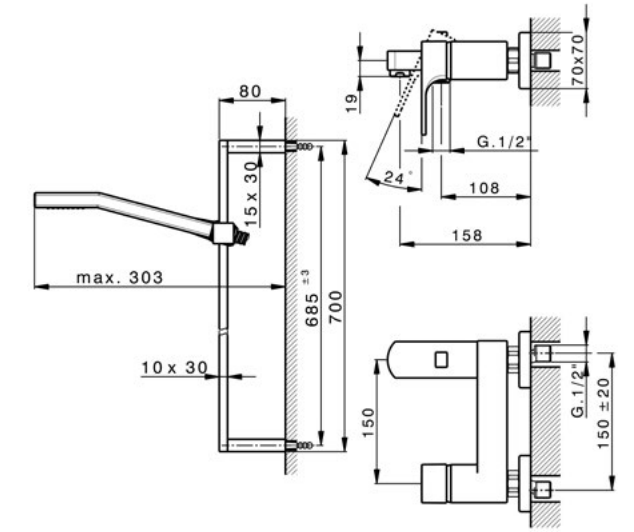
CU 00062 Completo Monocomando Vasca Bath/S. Mixer Set Ensemble Mitigeur Bain/D.
